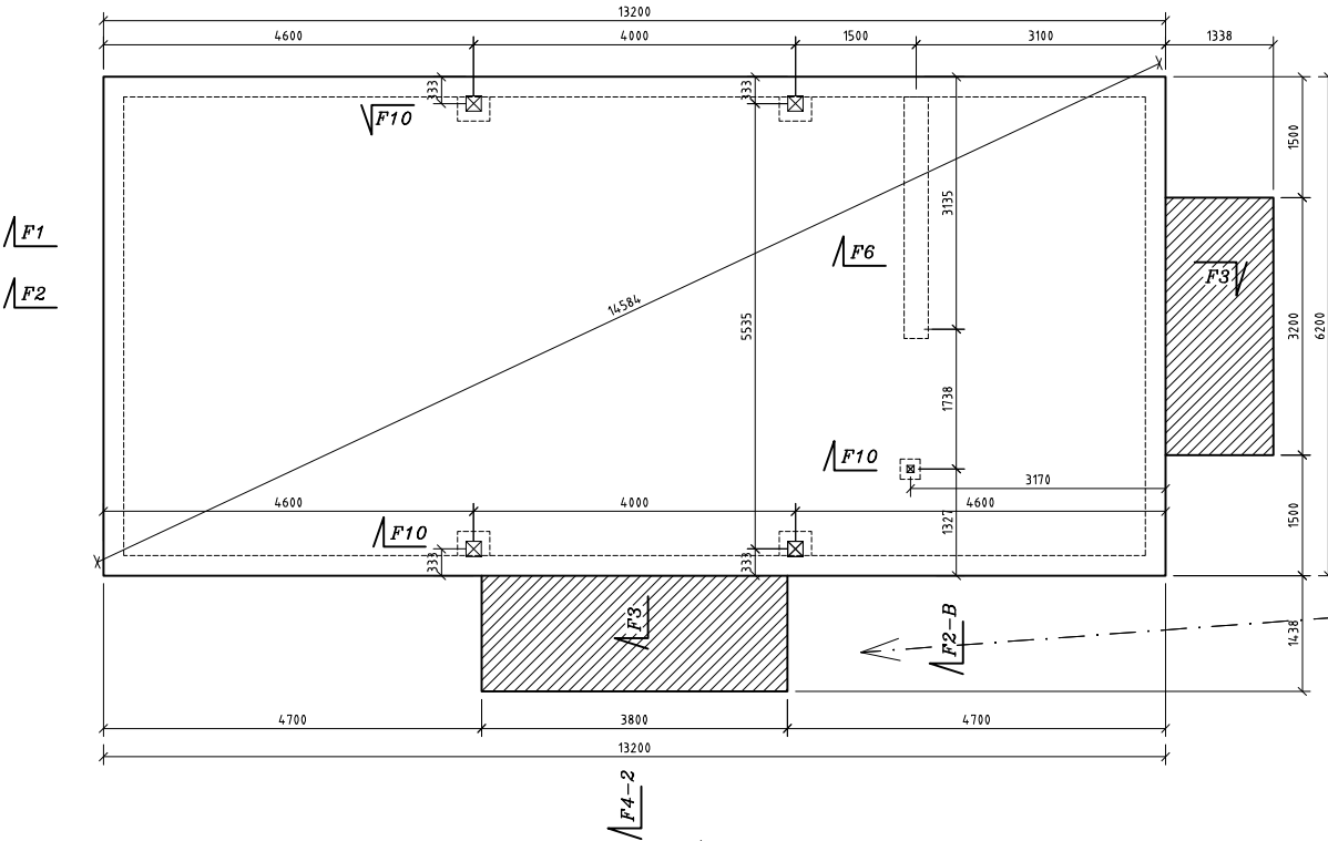
Foundation measures
