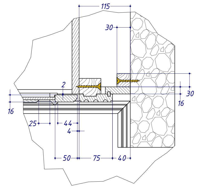
H (1:4)
