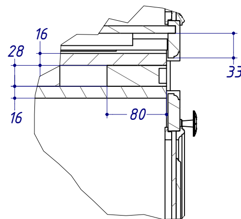
AP (1:5)
