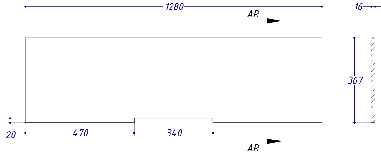
AR-AR (1:10)
