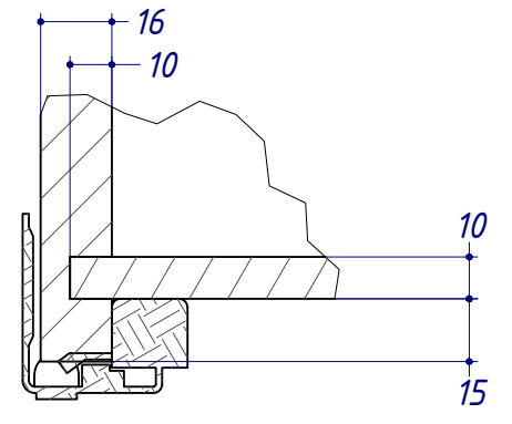
CW (1:2)
