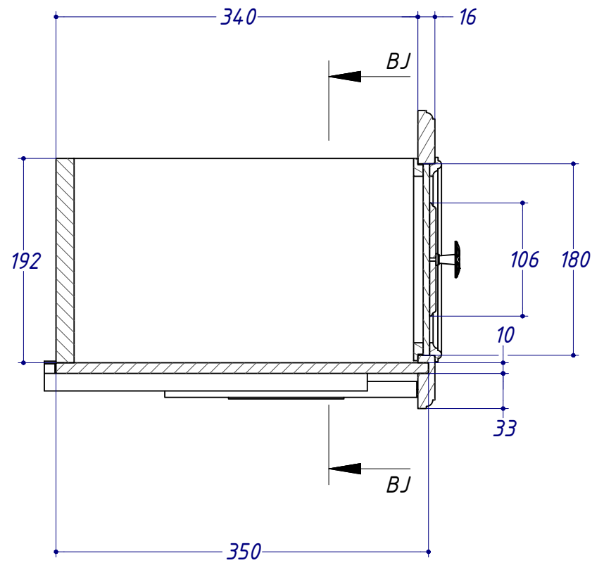
BG-BG (1:5)
