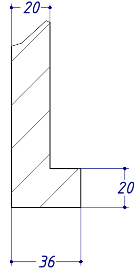
AW (1:2)
