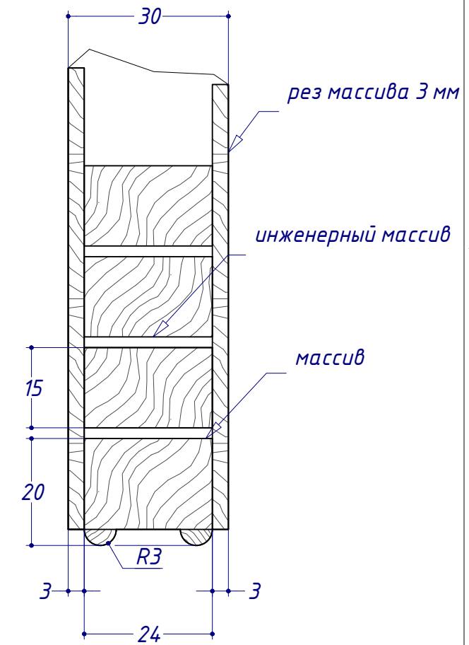
BB (1:1)
