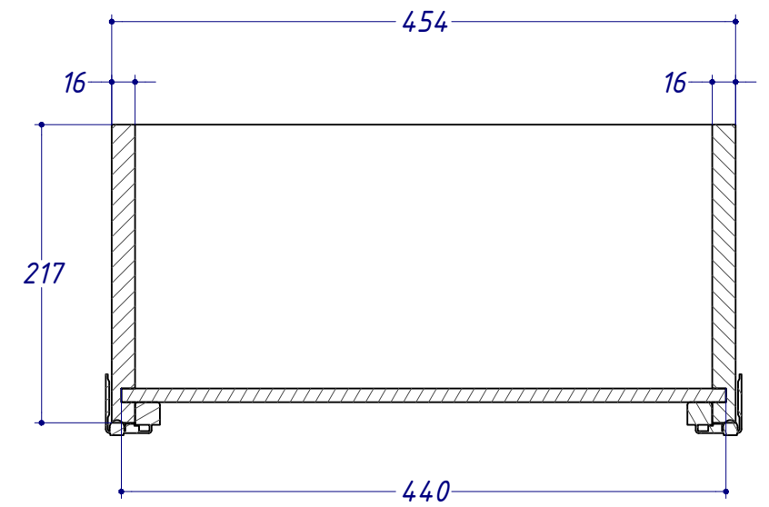
BE-BE (1:5)
